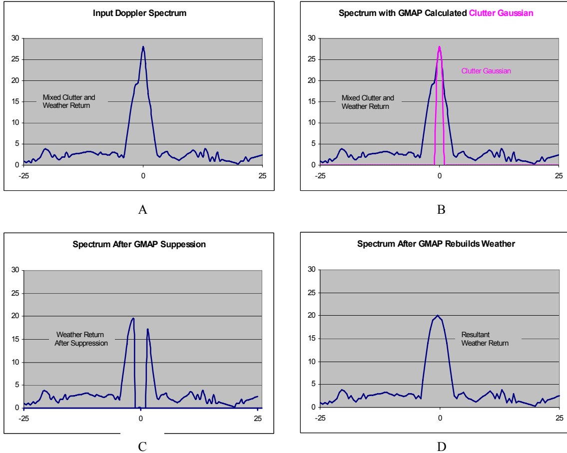
Figure 4. Conceptual Model of GMAP Clutter Filter with Return Centered Over Zero Velocity
