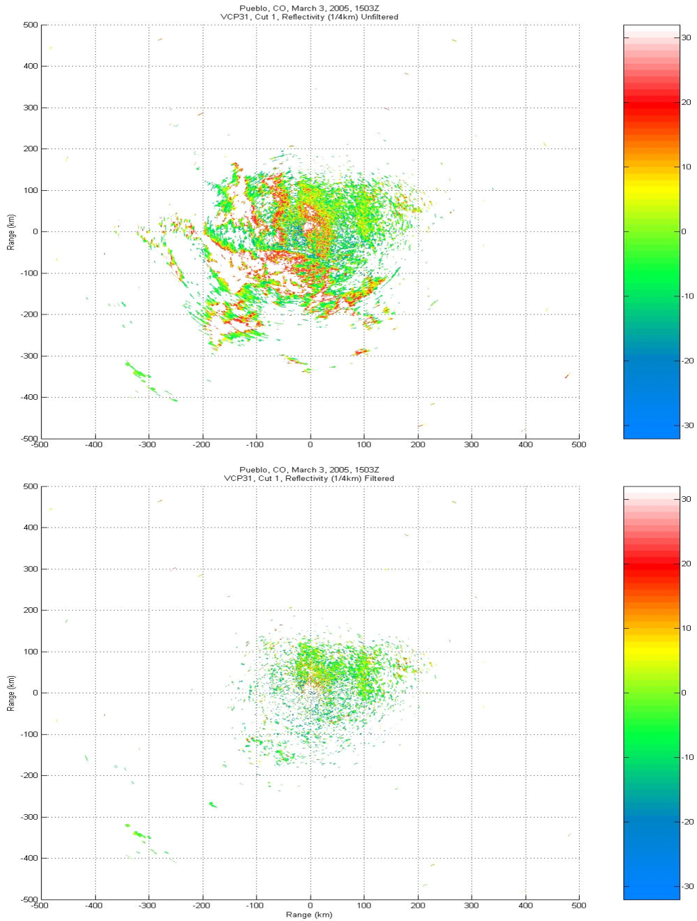
Figure 13. Reflectivity Without and With GMAP Clutter Suppression
