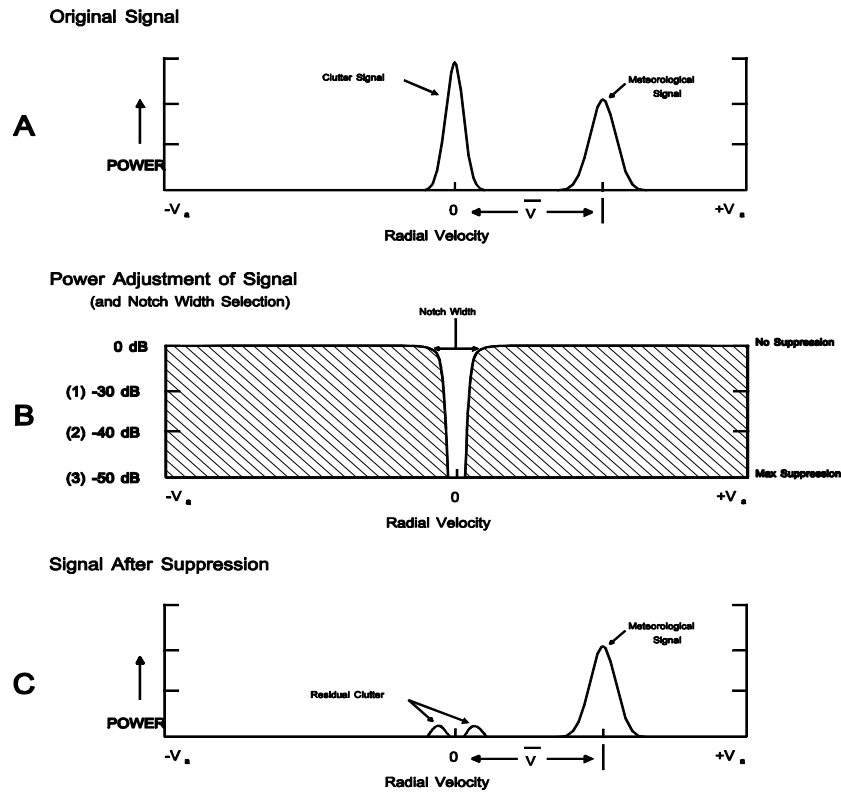
Figure 1. Simple Conceptual Model of Legacy Filter
