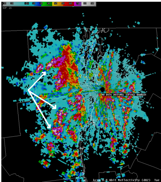
Figure 5. No clutter suppression
