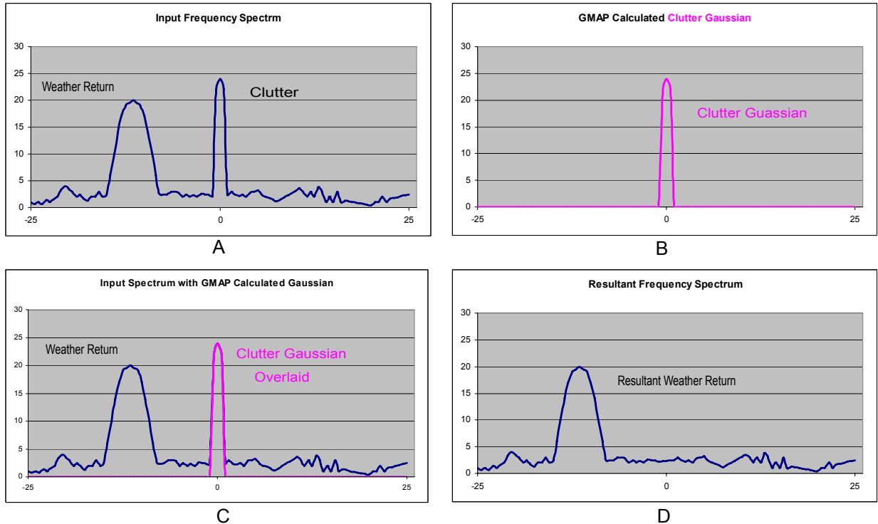
Figure 3. Conceptual Model of GMAP Clutter Filter
