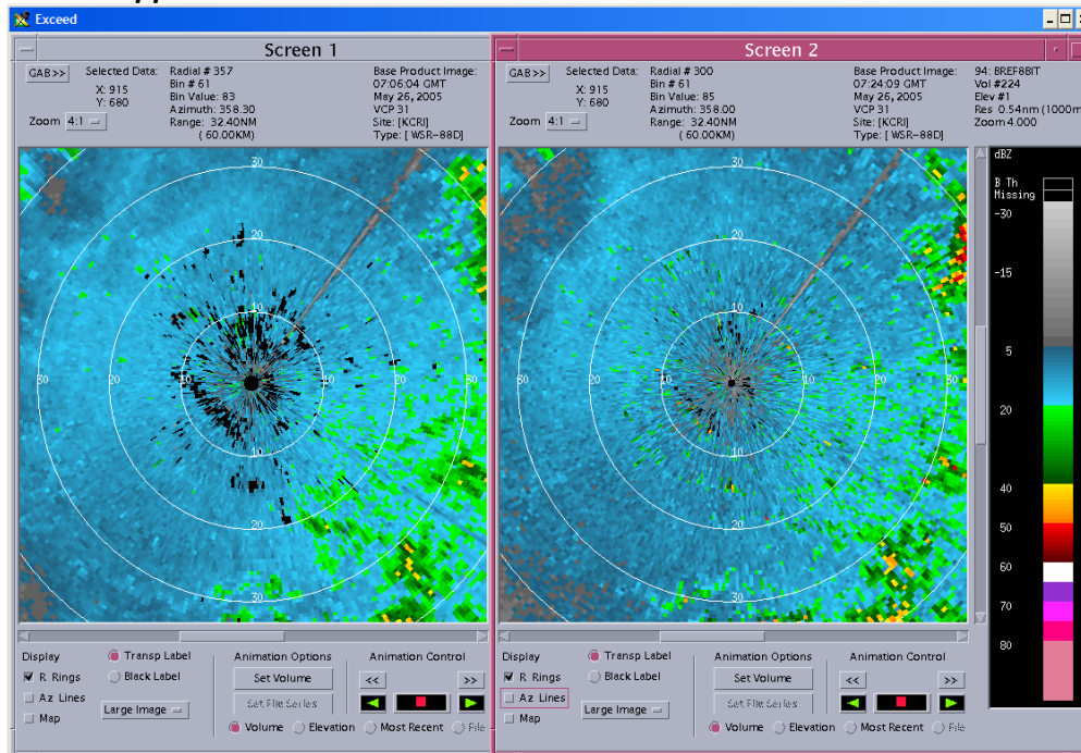
Figure 9. Legacy Clutter Censoring (Left) Verses ORDA Clutter Censoring (Right)
