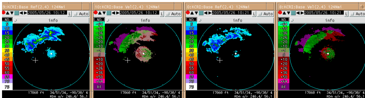
Figure 2. Example of Data Estimate Bias Caused by IIR Clutter Suppression
