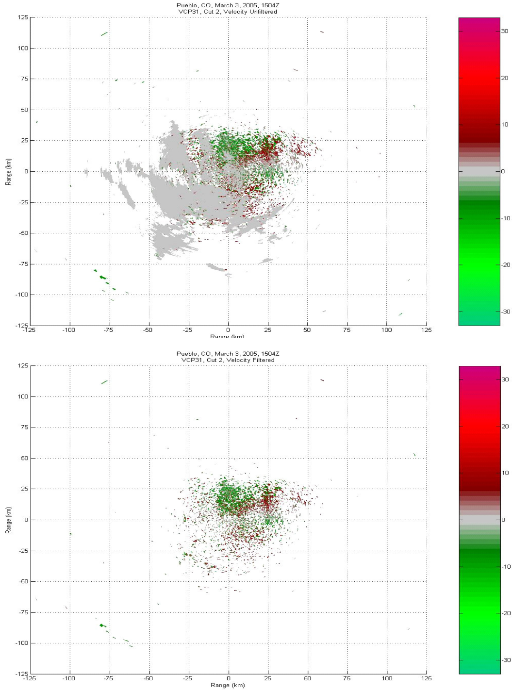
Figure 14. Velocity Data Without and With GMAP Clutter Suppression
