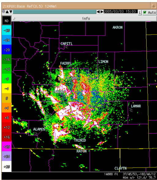
Figure 8. ORDA suppression in 2 zones
