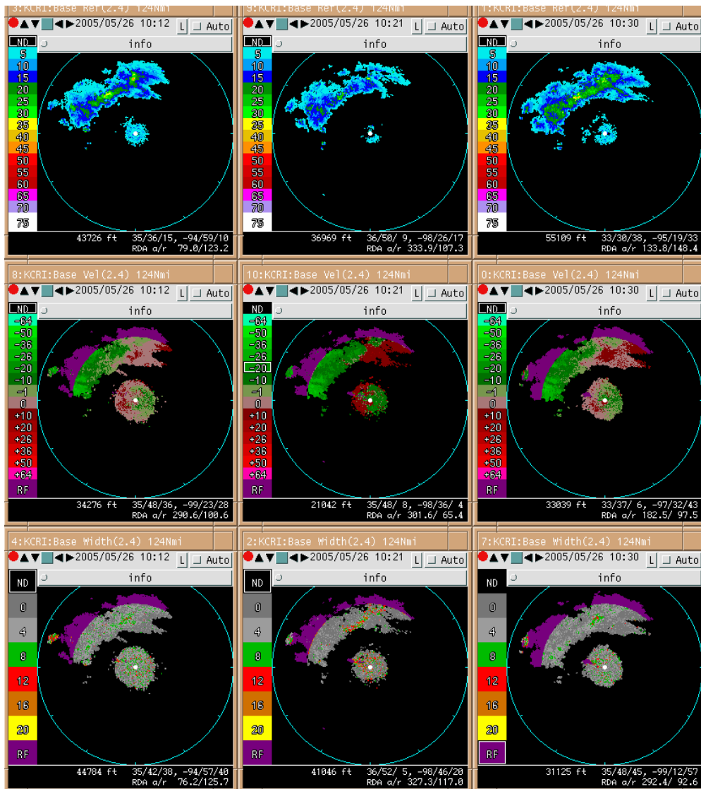
Figure 11. Example of Legacy Clutter Filter and GMAP Clutter Filter Induced Bias
