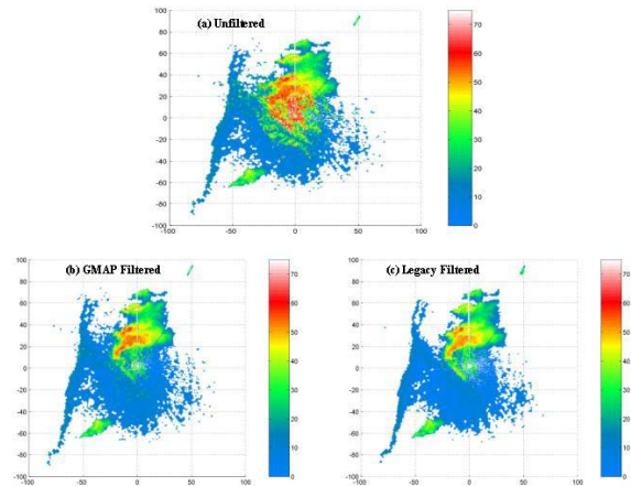
Figure 10 - May 8, 2003 Filter Comparison, Reflectivity
