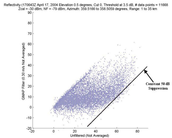
Figure 7 - Reflectivity Scatter gram - April 17, 2004
