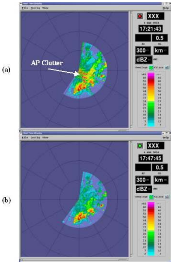
Figure 6 - KNQA AP Clutter Case 1997
