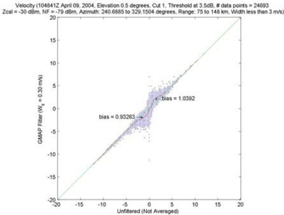
Figure 8 - Velocity Bias, Moderate Weather Returns
