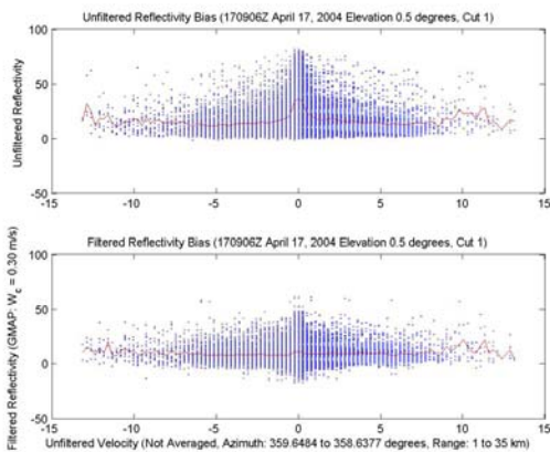
Figure 9 - Reflectivity Bias, Weak Meteorological Signal
