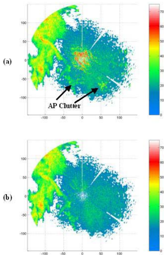
Figure 3 - Suppression - Convective Case, April 9, 2004
